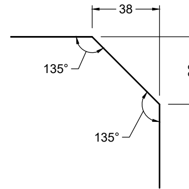
CHAMFER DETAIL
