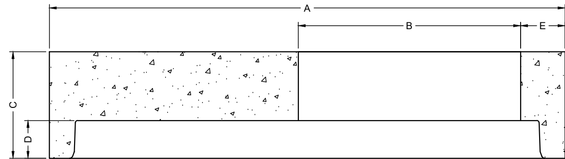
ELEVATION VIEW
