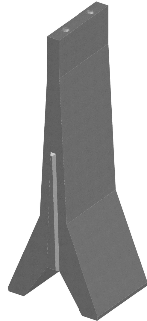
ISOMETRIC VIEW NTS
